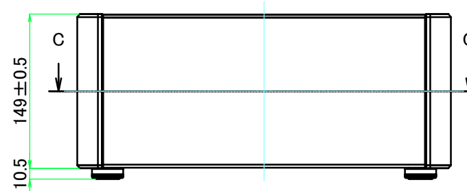
A view
